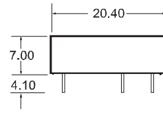
FXXXXD-1W Package
