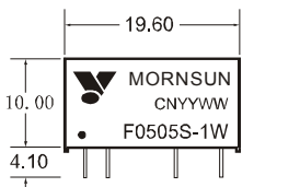
FXXXXS-1W Package
