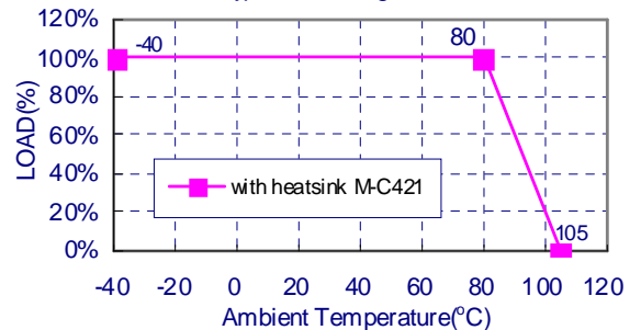
Typical Derating Curve
